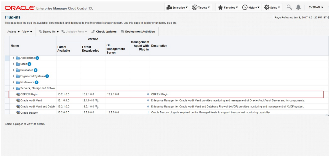
Figure 3–3 Select plug-in
